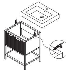
1. Paste the countertop Coller le comptoir
